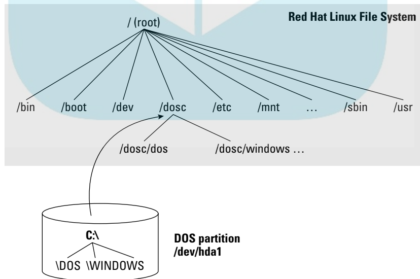
Figure 3-4: Here's how you mount a DOS partition on the /dosc directory.
